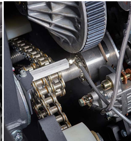
AUTO CHAIN LUBE SYSTEM 900-0112
